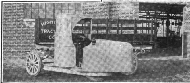
Above, tractor cab swung at right angles to allow traffic to pass ahead of it. Left, turning trailer in exact length of wheel-base of the semi-trailer. Right, cab and power plant reversed to run backward pushing the semi-trailer
